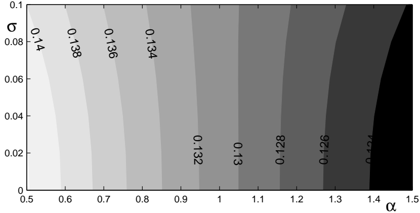
Figure 6: Optimal Emission control - Contour plot in the \alpha - \sigma space for high S and low K ([S,K]=[3500,500]).
