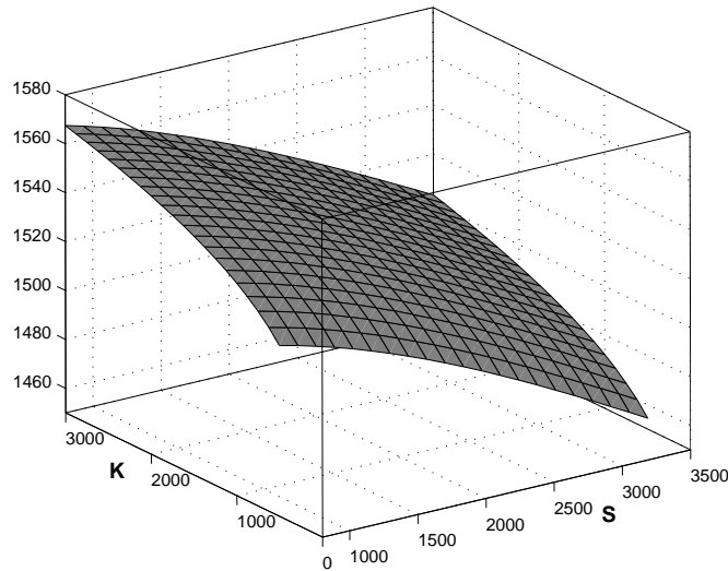
Figure 1: Value function
