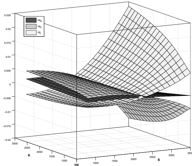
Figure 4: Difference in the shares of net output spent on emission control, Investment and consumption when uncertainty is included ( \Delta g_M, \Delta g_I, \Delta g_C ) respectively
