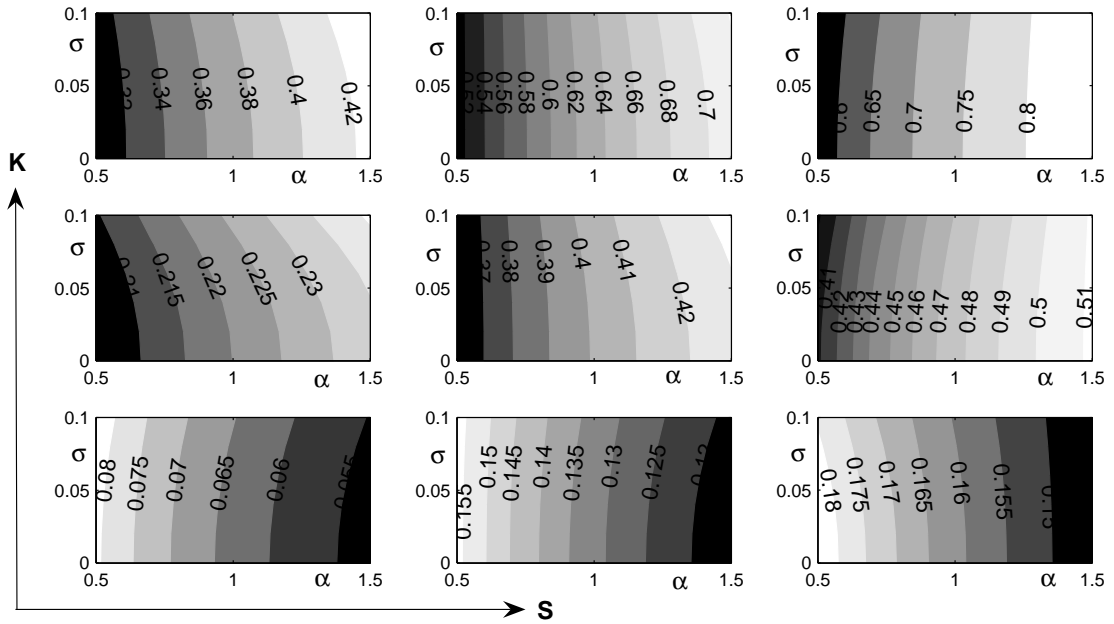
Figure 5: Optimal Emission control - Contour plots in the \alpha-\sigma space for combinations of S and K . S \in [800, 2150, 3500] and K \in [500, 1750, 3000] , with [S,K]=[800,500] in the lower left subplot.
