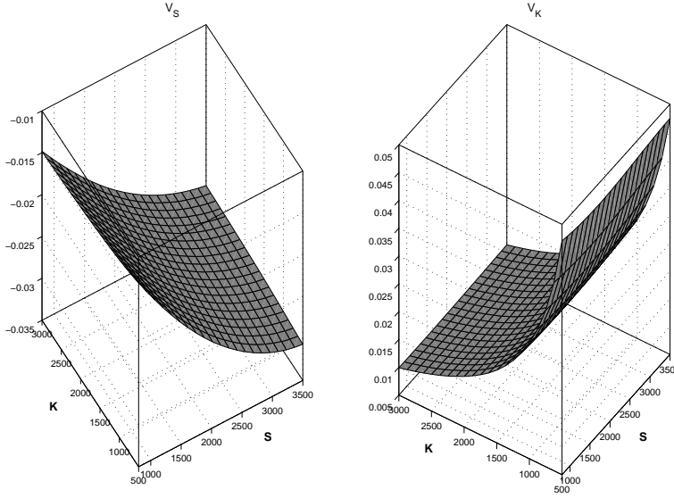
Figure 2: Shadow prices of atmospheric carbon stock ( \lambda_S ) and capital stock ( \lambda_K )
