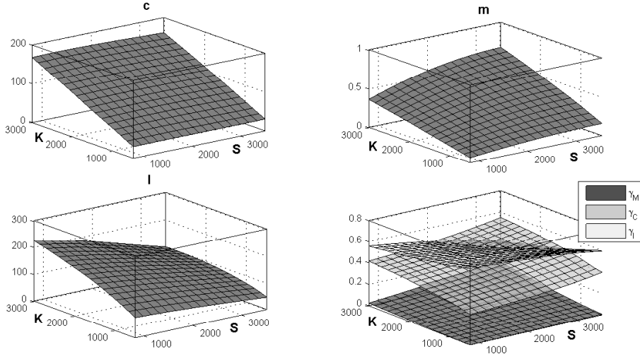
Figure 3: Policy functions for consumption ( c ), emission control ( m ), investment ( I ) and shares of net output spent on c , m and I
