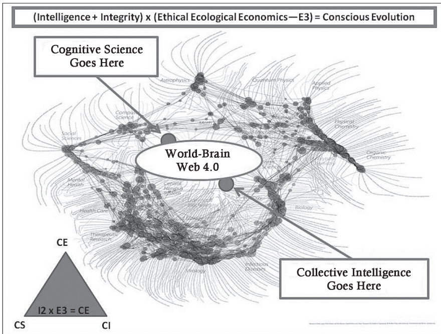
Figure 3. Scattered Knowledge.
