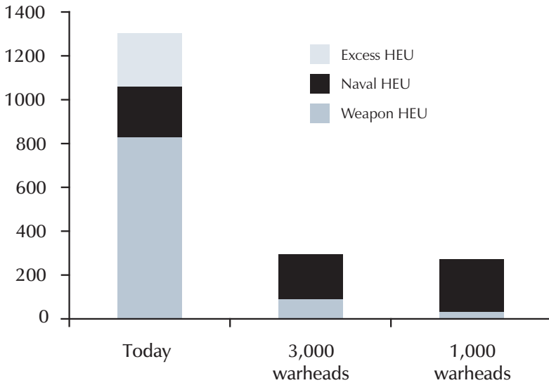
Figure 1. Global stockpiles of HEU in metric tons, today and in the future
