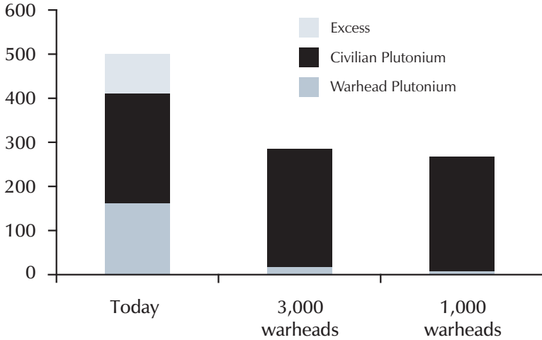
Figure 2. Global stockpiles of plutonium in metric tons, today and in the future
