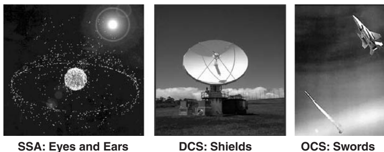
Figure 5. Counterspace operations
