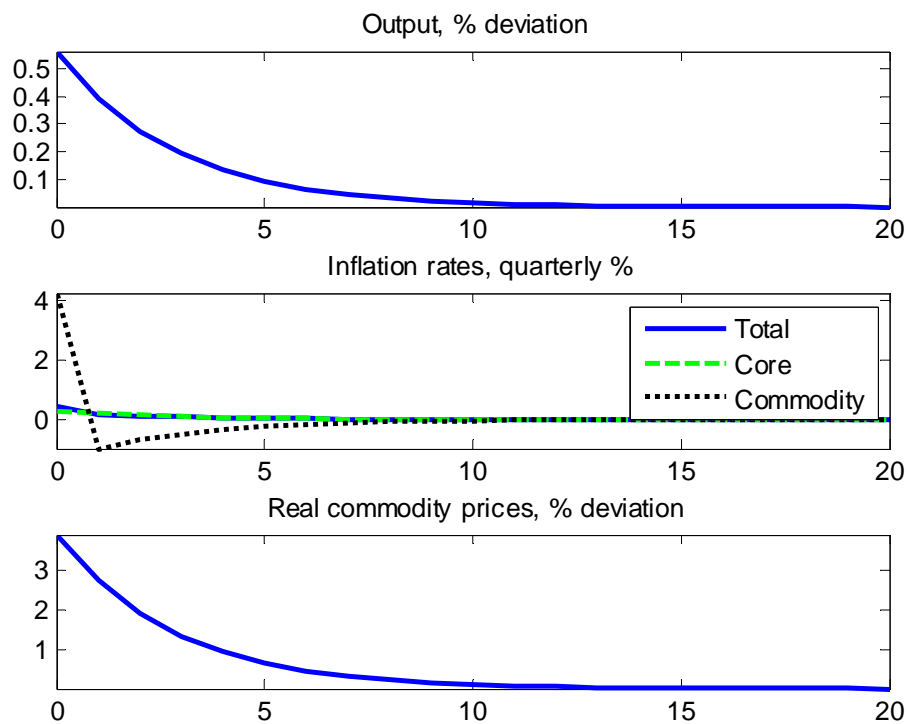
Figure 5: Impulse responses to a permanent 1% increase in nominal spending \gamma = 0.1 ; \phi = 0.1/1.1 ; \chi = 2 (Inelastic economy)
