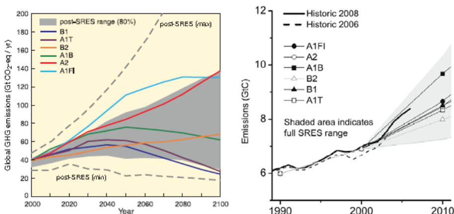
The present emission trajectory exceeds the ‘worst-case’ A1F1 IPCC scenario. Source: VanVuuren and Riahi 2008
