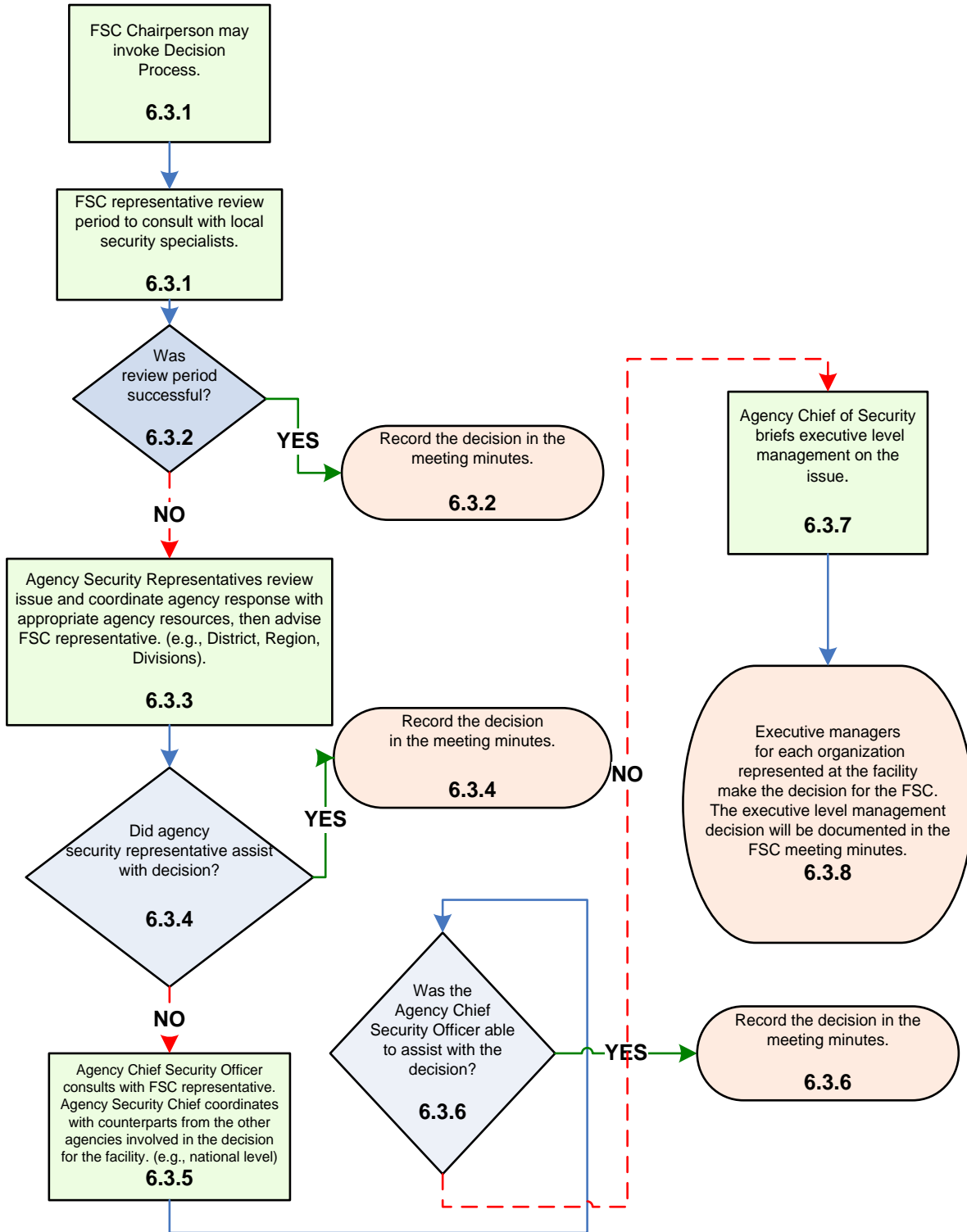
Figure 4: Decision Process
