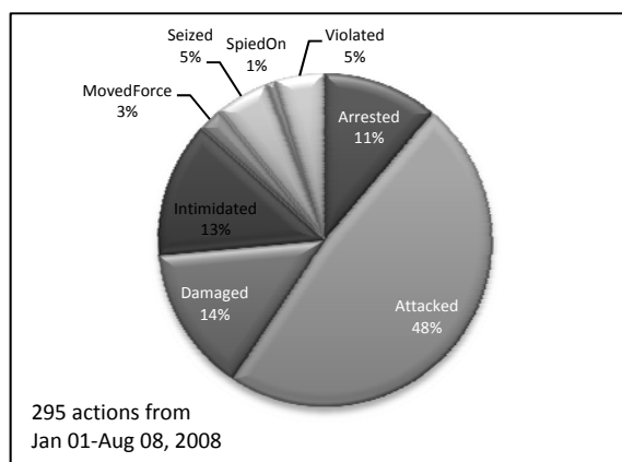
Figure 4 Hostile Actions
