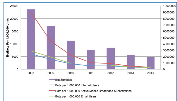
Figure 7: Botnets
