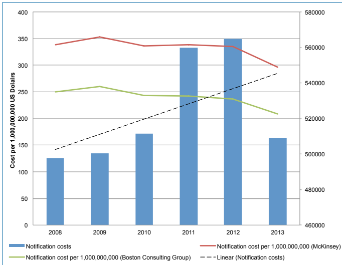
Figure 15: Notification Costs
