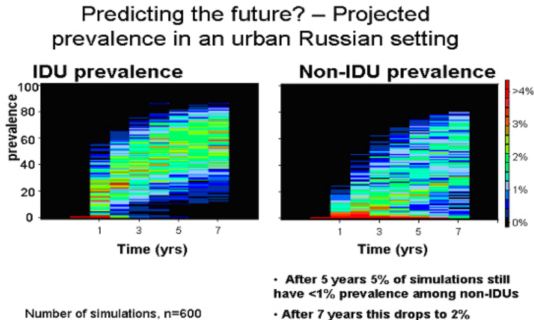
Figure 2.2: Monte-Carlo simulations of Russian HIV epidemic
