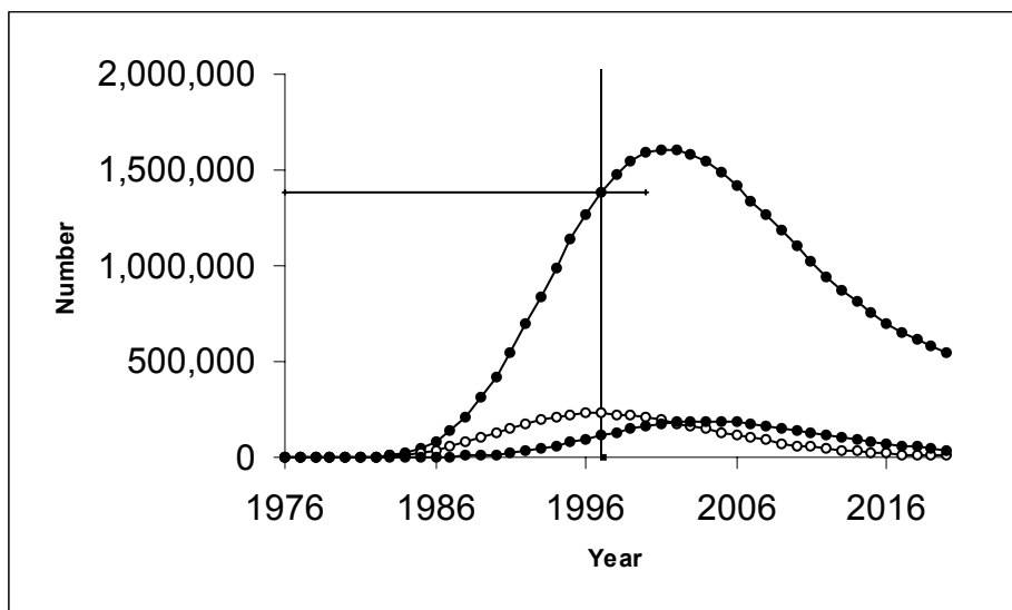
Figure A1.1 : An Epimodel AIDS epidemic
