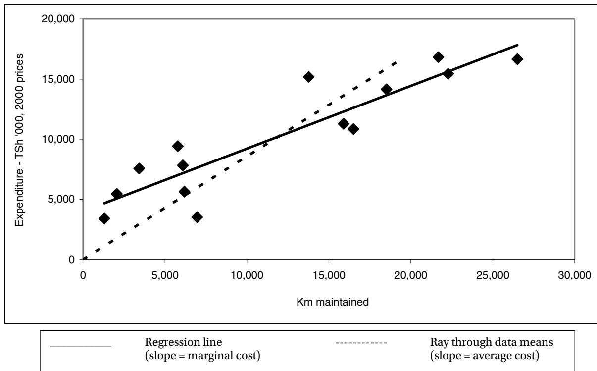
Fig. A2.10 Tanzania: Urban, district and feeder road maintenance 1992-2005
