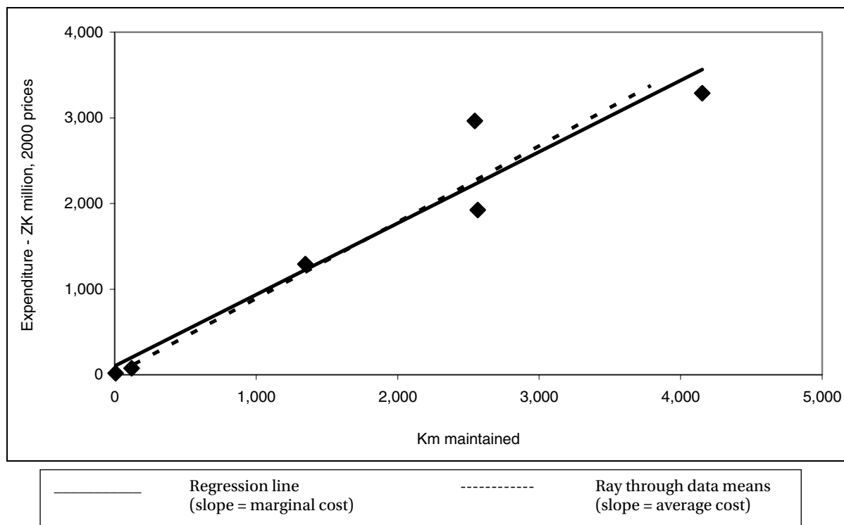
Fig. A2.15 Zambia: Non-urban, unpaved roads routine maintenance 2000-5
