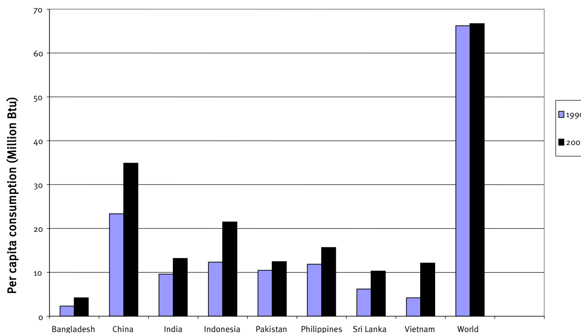
Figure 4: Average energy consumption, selected Asian economies and the World, 1990 and 2003
