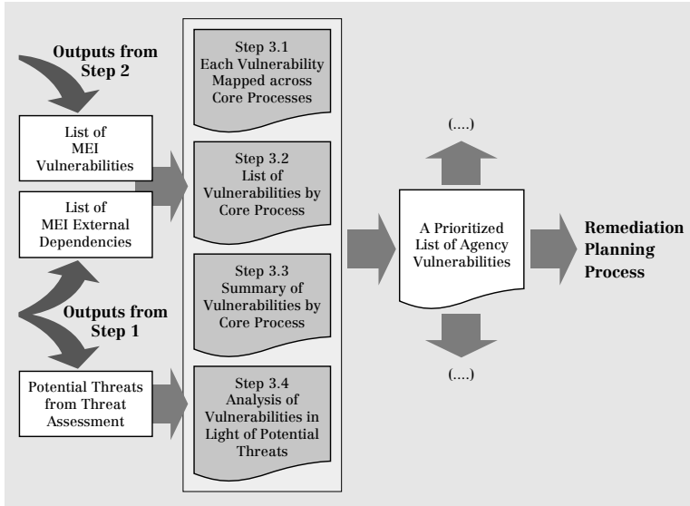
Figure 30: Step 3 Activities
